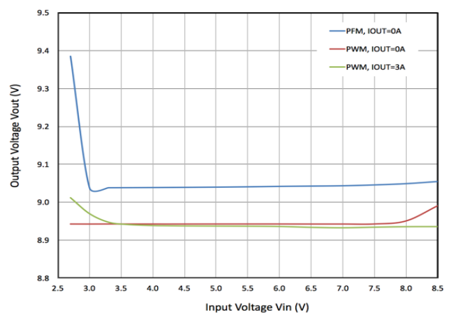
Figure 12. Line Regulation
