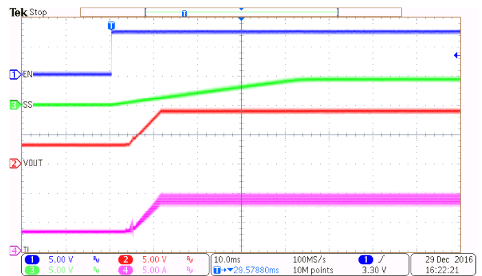
Figure 17. Power Up
