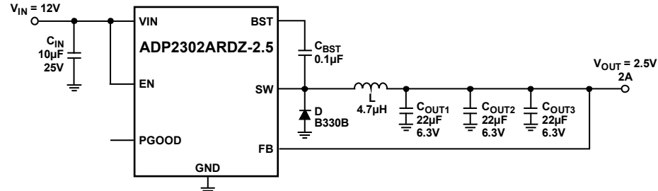
Figure 56. ADP2302 Typical Application, V_{IN} = 12V , V_{OUT} = 2.5V , 2A
