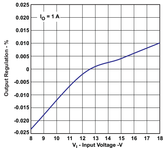
Figure 16. TPS54233 Line Regulation
