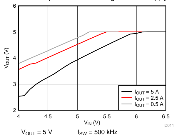
Figure 7. Dropout Curve
