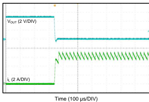
Figure 28. Output Short
