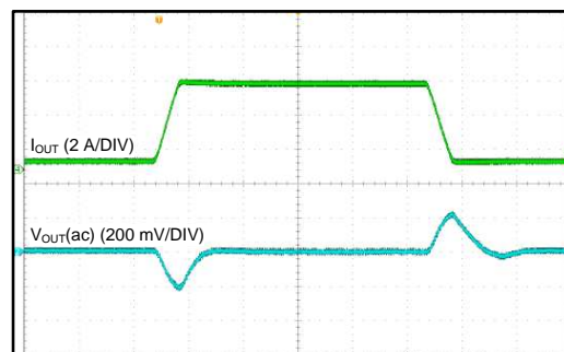
Figure 25. DCM Mode
