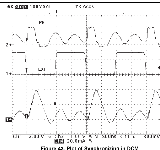
Figure 43. Plot of Synchronizing in DCM
