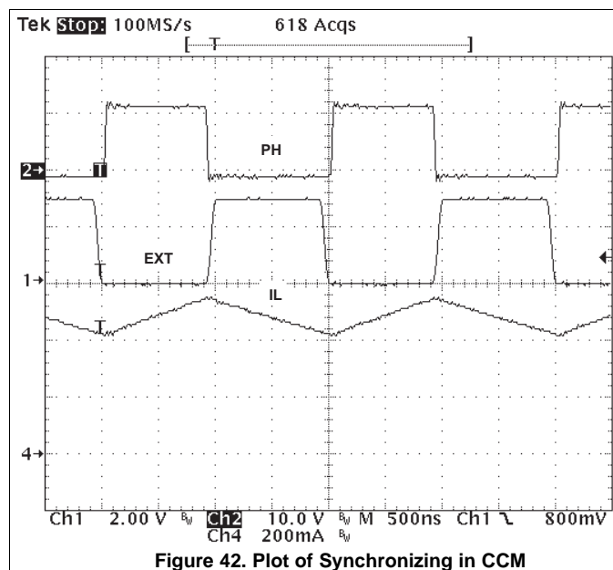
Figure 42. Plot of Synchronizing in CCM
