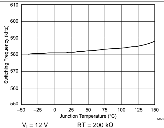
Figure 4. Switching Frequency vs Junction Temperature
