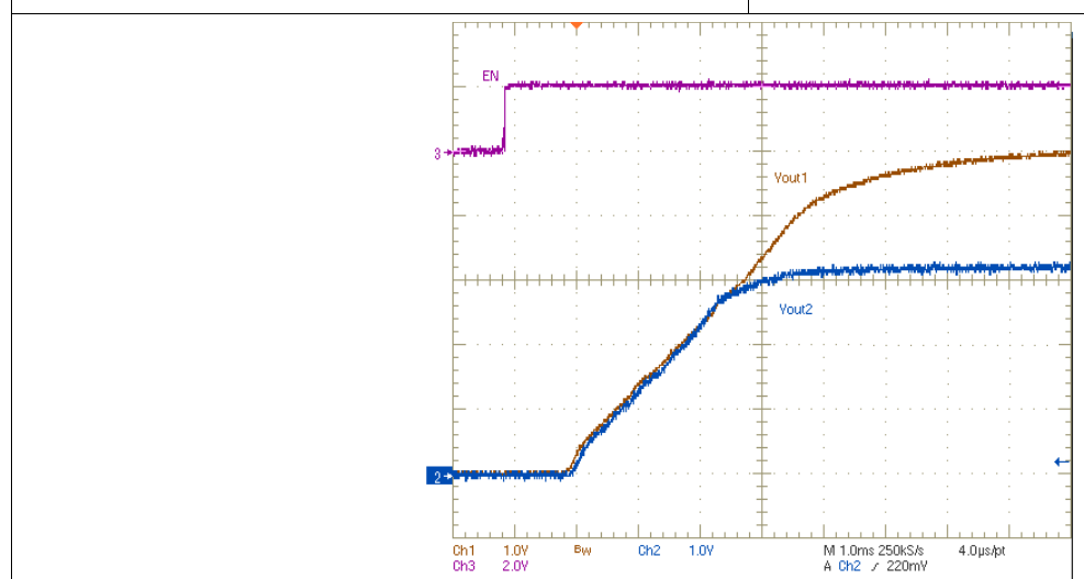
Figure 36. Simultaneous Startup With Tracking Resistor
