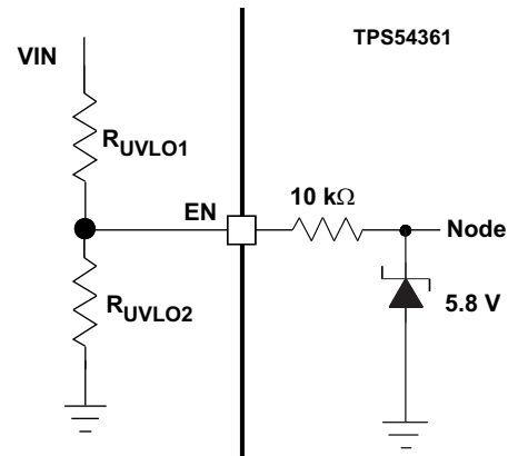
Figure 27. Internal EN Pin Clamp
