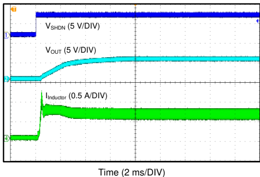
Figure 10. Start-up Waveform
