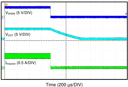
Figure 11. Shutdown Waveform
