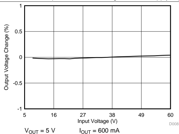
Figure 7. Line Regulation
