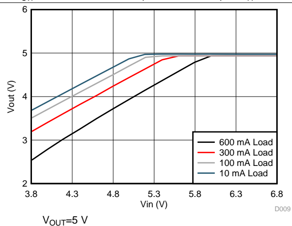
Figure 8. Dropout Curve
