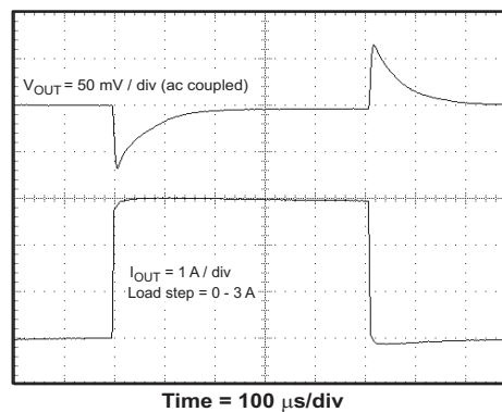
Figure 35. Transient Response
