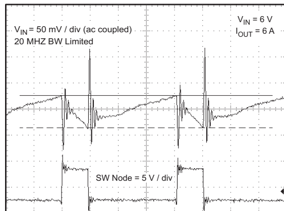
Figure 40. Input Ripple
