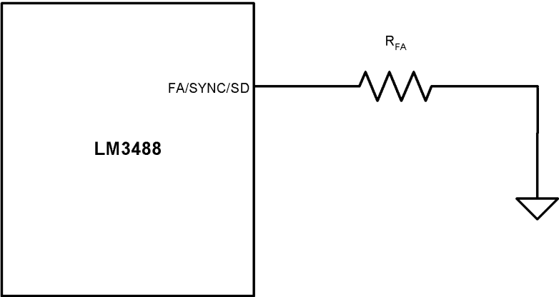
Figure 25. Frequency Adjust
