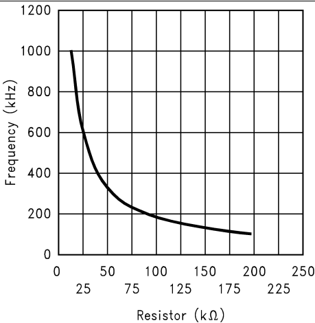
Figure 4. Switching Frequency vs RFA
