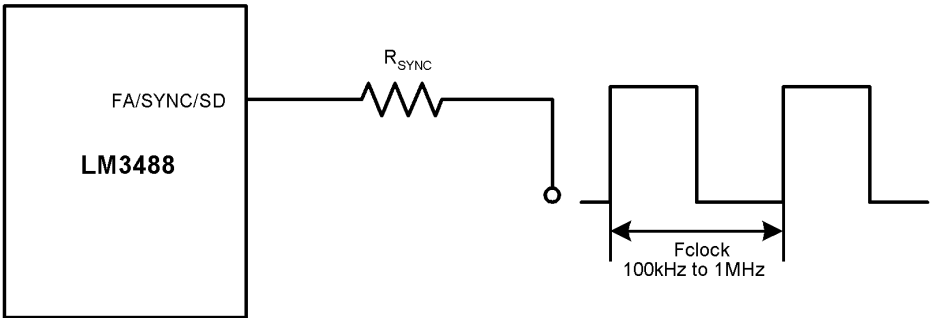
Figure 26. Frequency Synchronization
