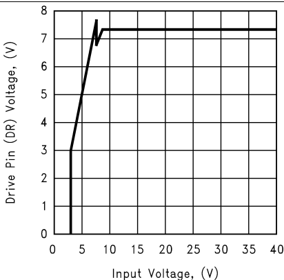
Figure 6. Drive Voltage vs Input Voltage
