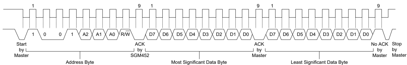
(a) Typical 2-Byte Read from Preset Pointer Location Such as Temperature, T_{OS} , T_{HYST}
