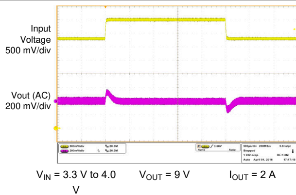
Figure 9-8. Line Transient
