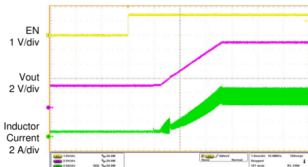
Figure 9-5. Start-up Waveforms
