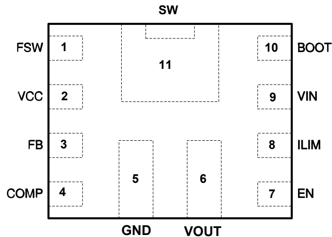
Figure 6-1. 11-Pin VQFN With Thermal Pad RNR Package (Top View)
