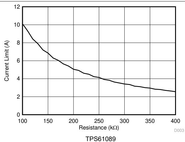
Figure 7-3. Switching Peak Current Limit Setting
