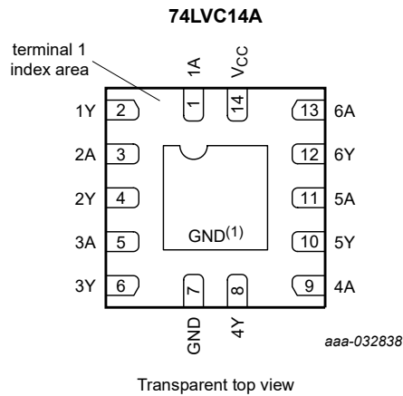
Fig. 6. Pin configuration SOT8014-1 (DHXQFN14)
