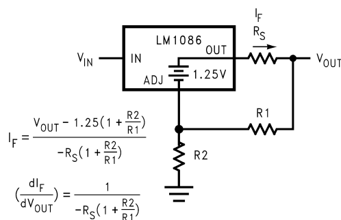
Figure 21. Battery Charger
