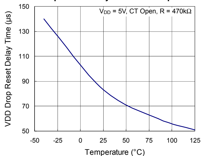
VDD Drop Reset Delay Time vs. Temperature
