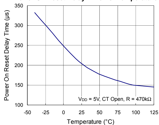
Power On Reset Delay Time vs. Temperature
