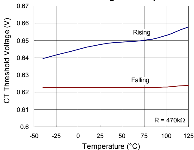
CT Threshold Voltage vs. Temperature
