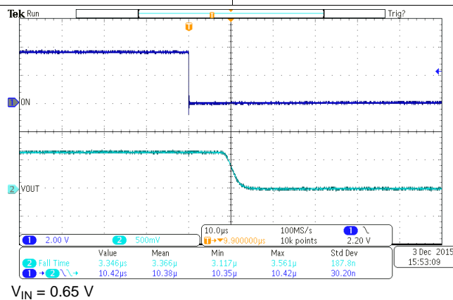
Figure 29. Turnoff Response (TPS22925xx)
