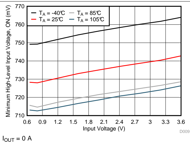
Figure 11. High-Level Input Voltage vs Input Voltage
