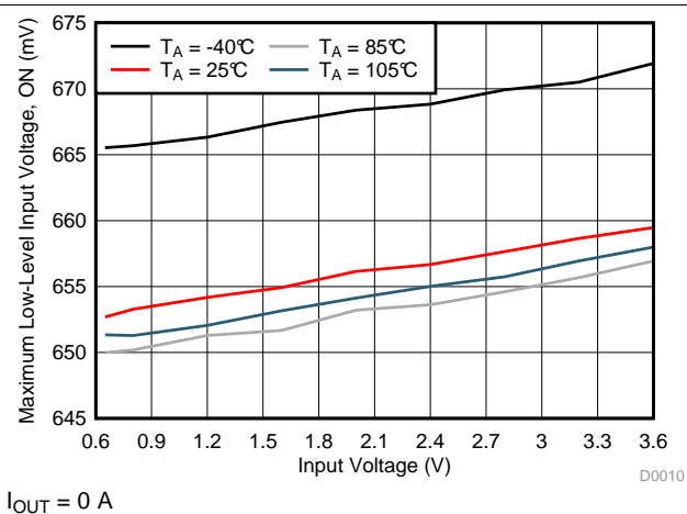
Figure 12. Low-Level Input Voltage vs Input Voltage
