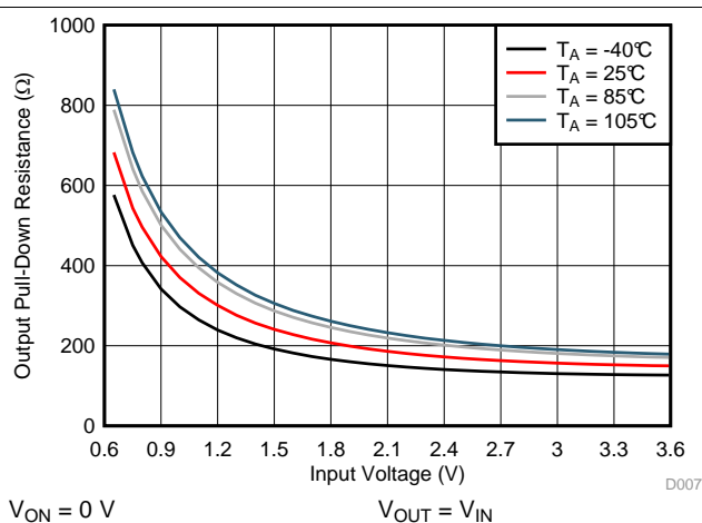
Figure 9. Output Pull-Down Resistance vs Input Voltage
