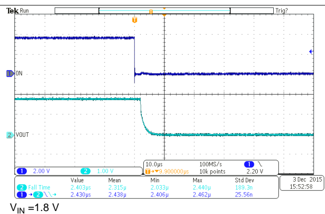
Figure 28. Turnoff Response (TPS22925xx)
