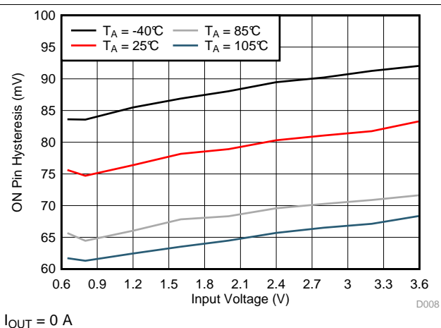
Figure 10. Hysteresis vs Input Voltage
