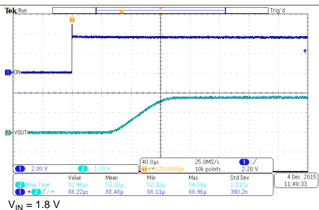
Figure 22. Turnon Response (TPS22925Bx)
