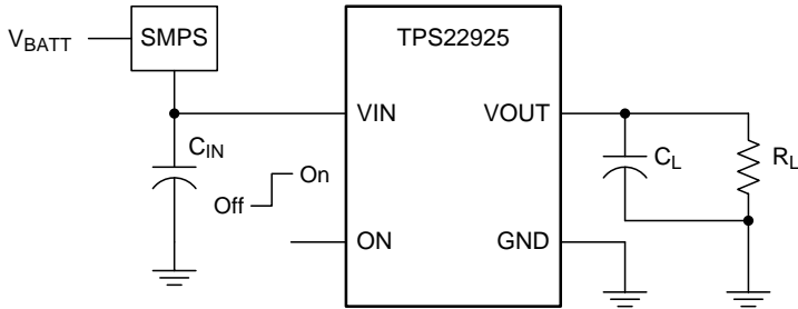
Figure 33. Typical Application Schematic
