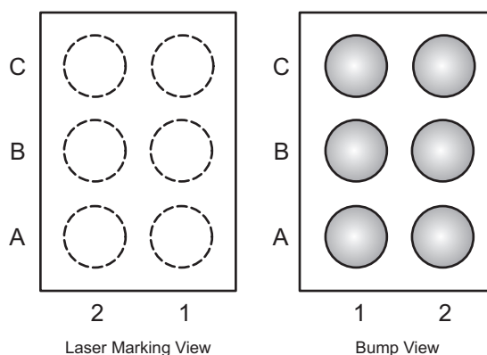
Pin Assignments
