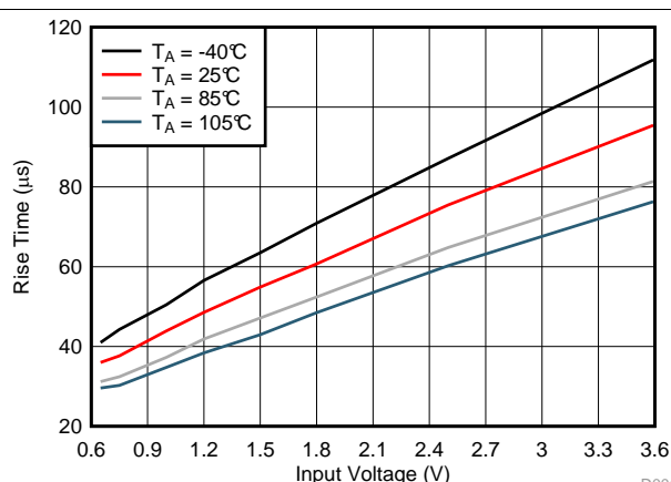
Figure 16. Rise Time vs Input Voltage (TPS22925Bx)
