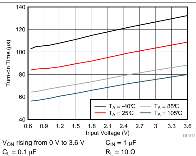
Figure 13. Turn-on Time vs Input Voltage (TPS22925Bx)
