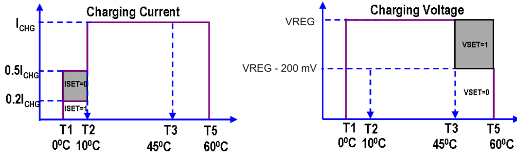
Figure 15. Charging Values
