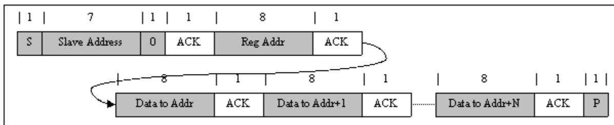
Figure 23. Multi-Write
