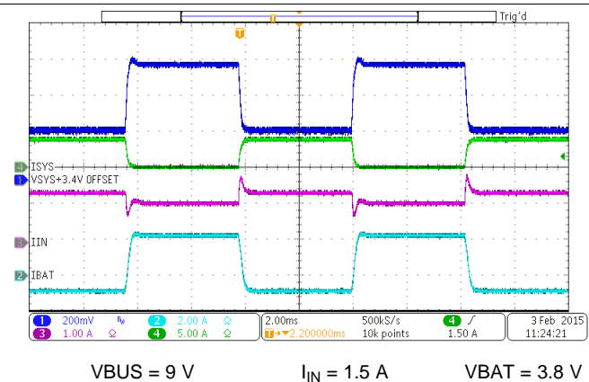
Figure 51. Charge Disable
