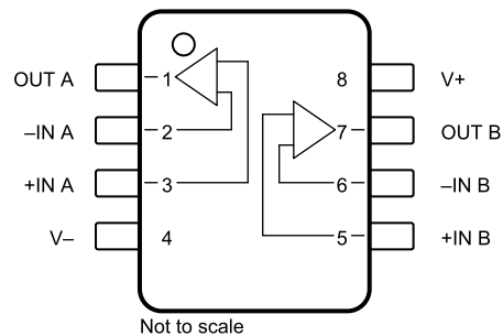
OPA2314-Q1 DGK Package 8-Pin VSSOP Top View
