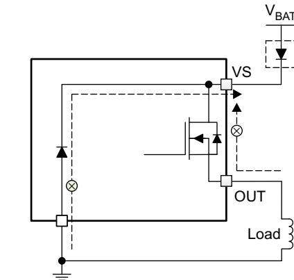
Figure 33. Reverse-Current External Protection, Method 1
