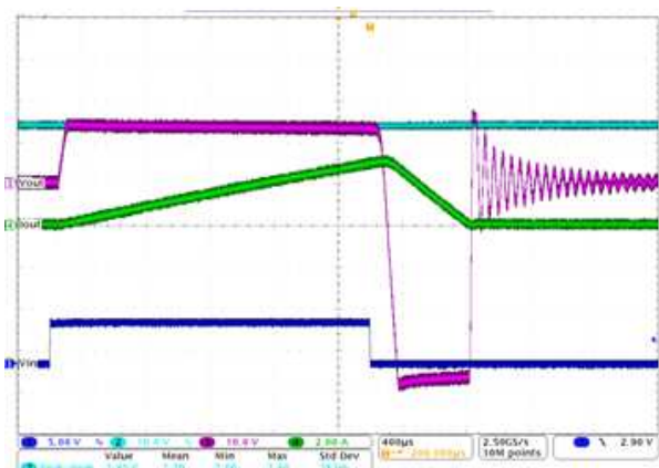
Figure 26. Inductive Load Switching-Off Waveform
