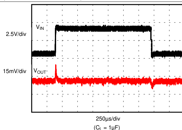
Figure 14. Line Transient
