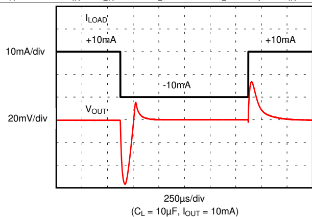
Figure 13. Load Transient
