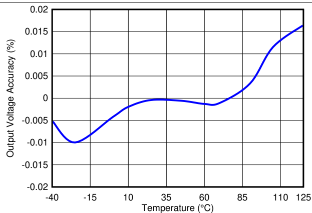
Figure 1. Temperature Drift
