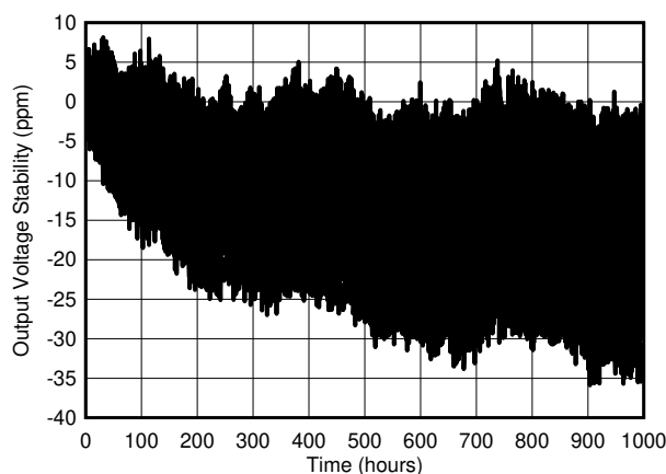
Figure 23. Long Term Stability - 1000 hours ( V_{REF} )
