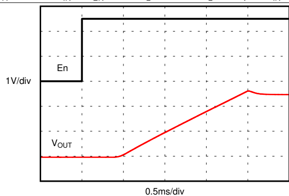
Figure 19. Turnon Time (Enable)
