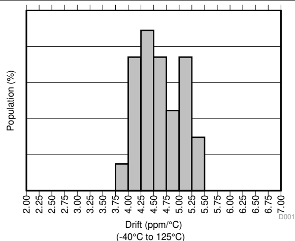
Figure 1. Temperature Drift
