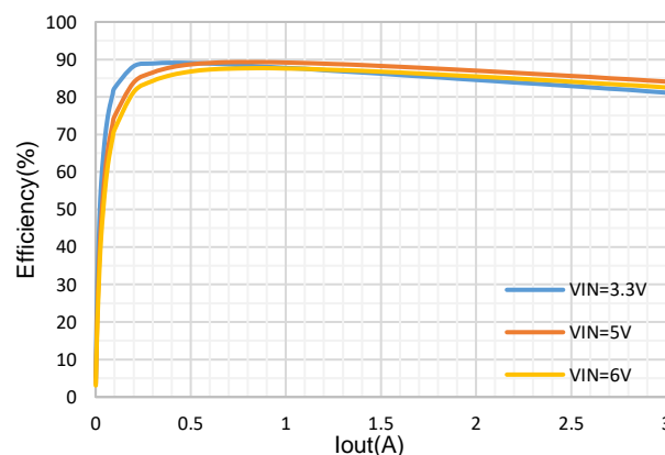
Efficiency, Vout=1.2V
