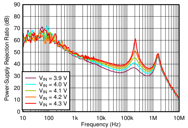
Figure 5-32. PSRR vs Frequency and V_{IN}
