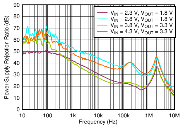
Figure 5-34. PSRR vs Frequency and V_{IN}
