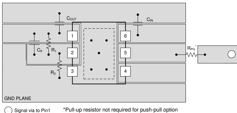
Figure 7-11. Layout Example for the DRV Package
