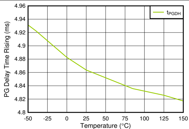
Figure 5-19. t_{PGDH} vs Temperature (For TPS746B Only)
