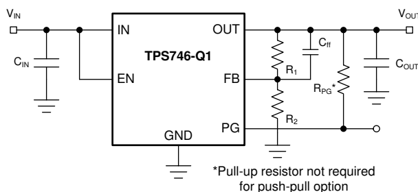
Figure 7-9. TPS746-Q1 Typical Application
