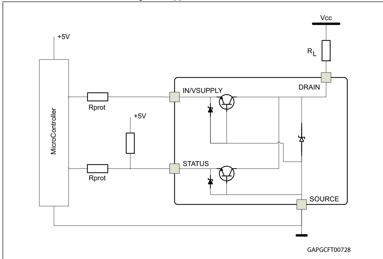
Figure 5. Application schematic
